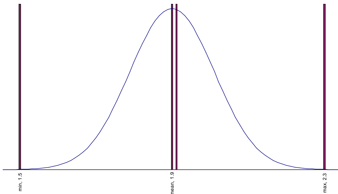
Figure: plot of the distribution of lead in the 1,000 units, with minimum concentration of 1.5 mg/kg, mean concentration in the lot of 1.9 mg/kg and maximum concentration of 2.3 mg/kg. The specification limit is 2 mg/kg.
